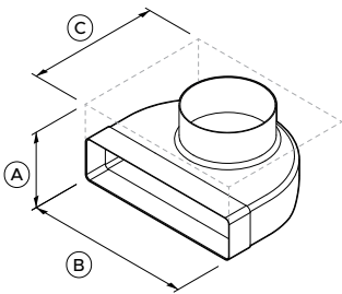
4 Duct Adapter 90°, 300x70 Rectangular to Round
