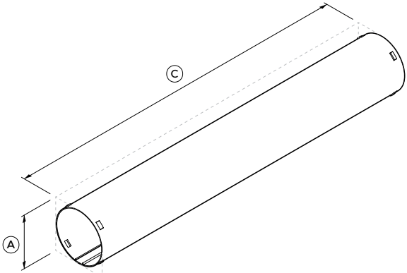
8 Duct Straight Length 1m, Round, 150
