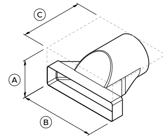
3 Straight Adapter, 300x70 Rectangular to Round
