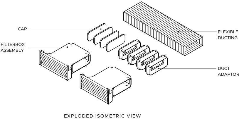
EXPLODED ISOMETRIC VIEW
