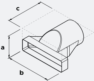
3 Straight Adapter, 300x70 Rectangular to Round
