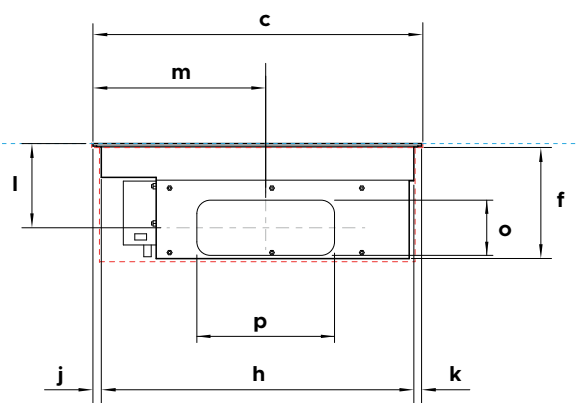
PROFILE VIEW
