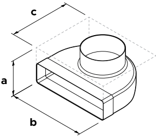
4 Duct Adapter 90°, 300x70 Rectangular to Round
