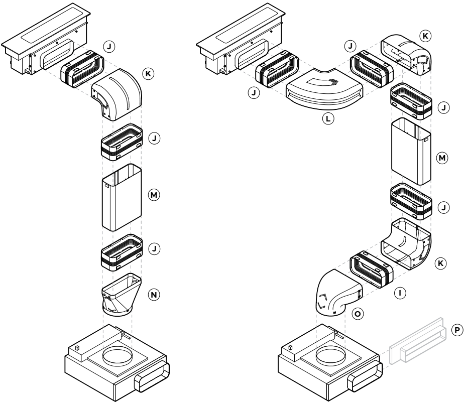
CD13DB2 CD13DG2 MODULAR VENTILATION - 222 X 89 DUCTING
