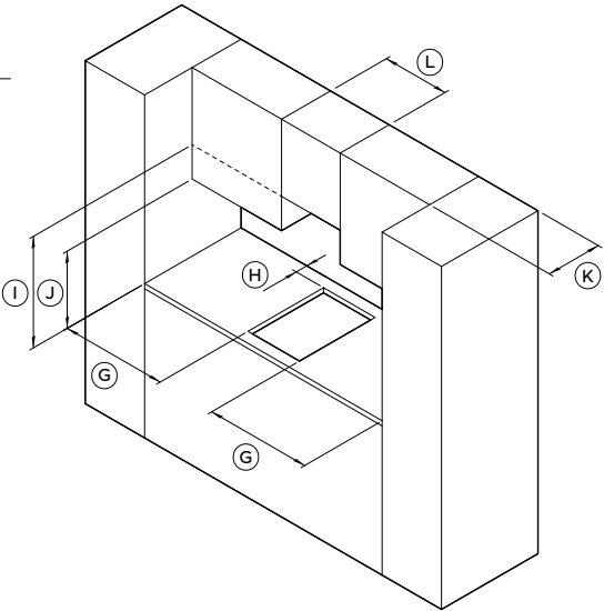
CLEARANCE OVERVIEW
