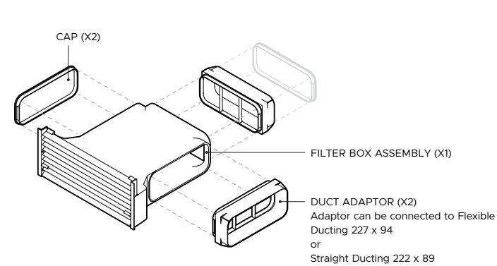
EXPLODED ISOMETRIC VIEW
