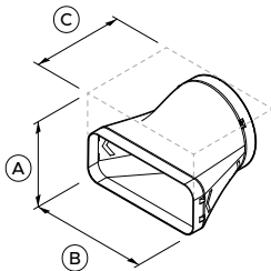
3 Adapter Straight, 150 to 222x89
