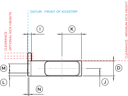
PROFILE VIEW
