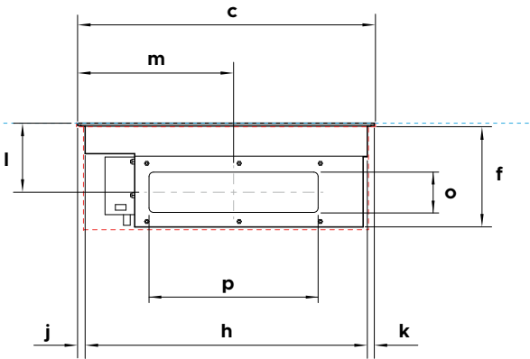
PROFILE VIEW
