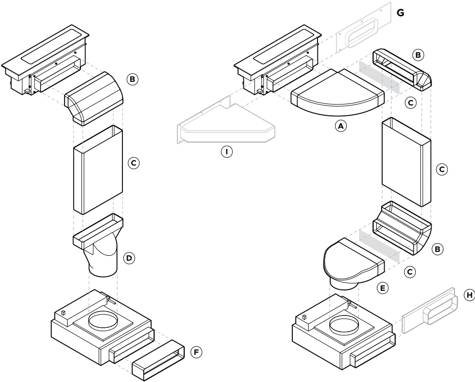
CD13DB1 CD13DG1 MODULAR VENTILATION - 300 X 70 DUCTING
