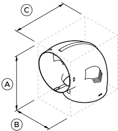
⑥ 90° Bend, Round 150
