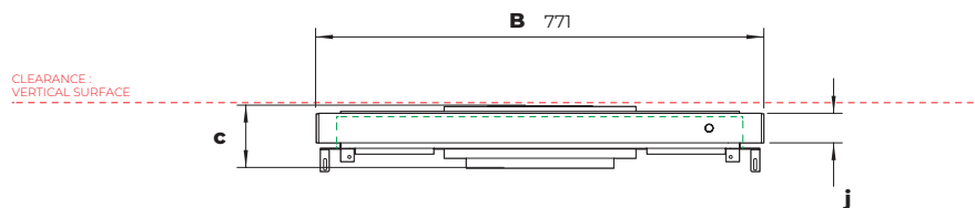
PLAN VIEW
