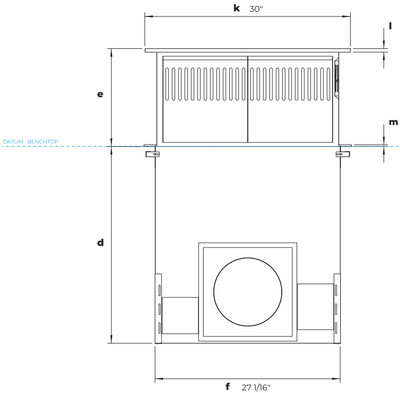
FRONT VIEW
