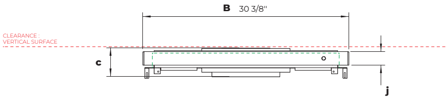
PLAN VIEW
