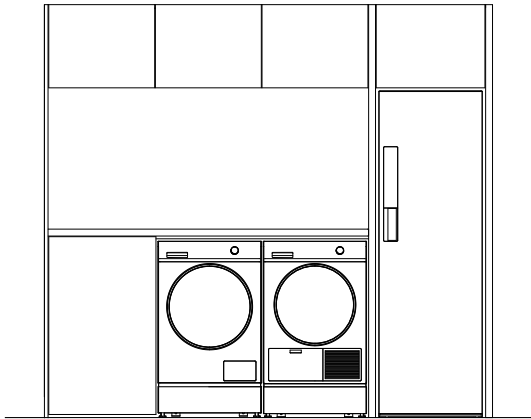
④ SIDE BY SIDE WITH PLINTHS AND FABRIC CARE CABINET
