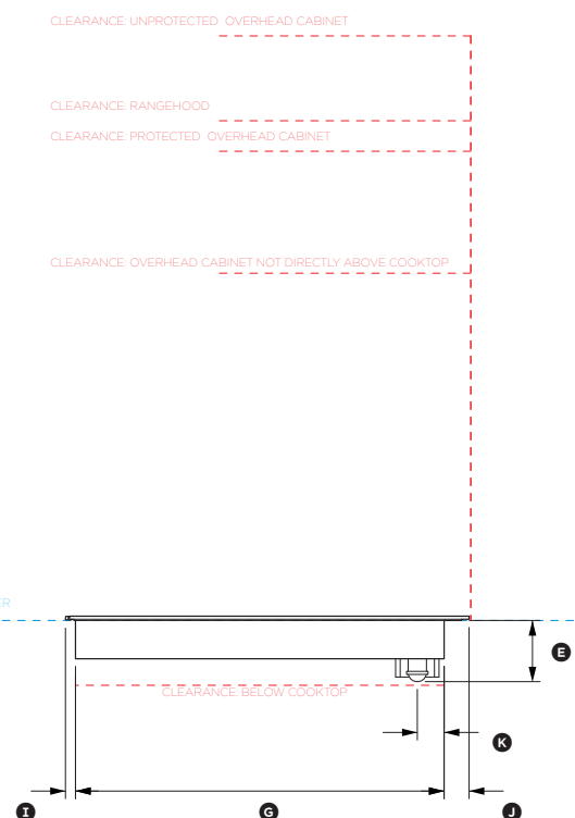
PROFILE VIEW
