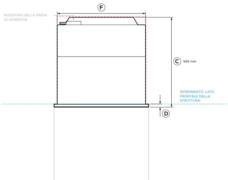
VISTA IN PIANO
