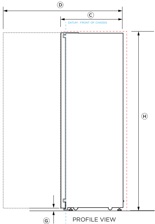
PROFILE VIEW
