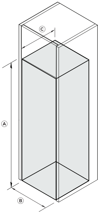
ISOMETRIC VIEW
