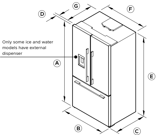
ISOMETRIC VIEW
