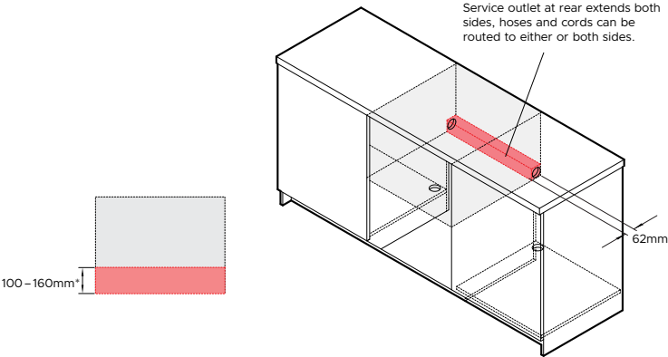
REAR VIEW
