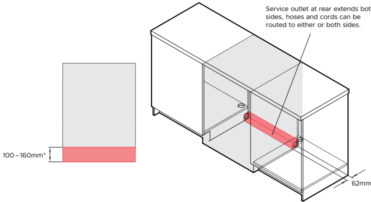
REAR VIEW
