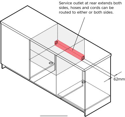
ISO VIEW
