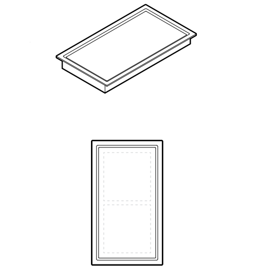
AUXILIARY MODULAR TEPPANYAKI COOKTOP, 12", 2 ZONES
