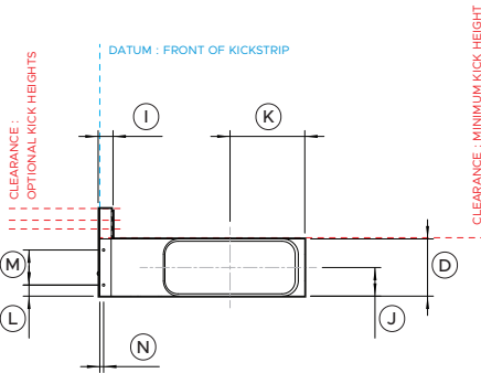
PROFILE VIEW
