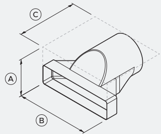
③ Straight Adapter, 300x70 Rectangular to Round
