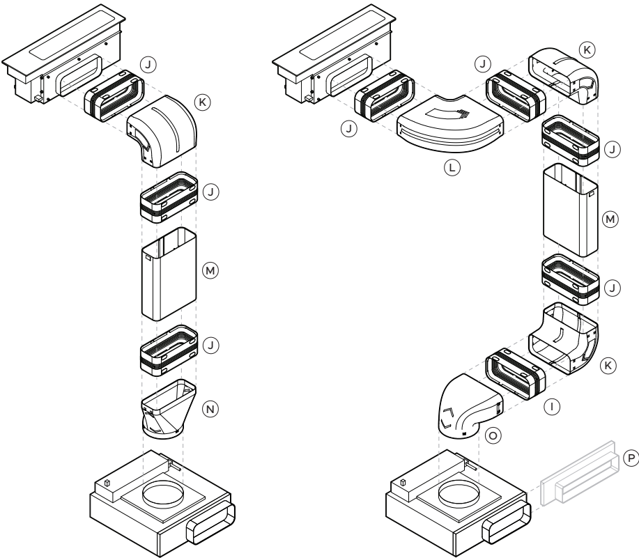
CD13DB2 CD13DG2 MODULAR DOWNDRAFT - 222 X 89 DUCTING
