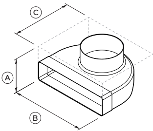
④ Duct Adapter 90°, 300x70 Rectangular to Round
