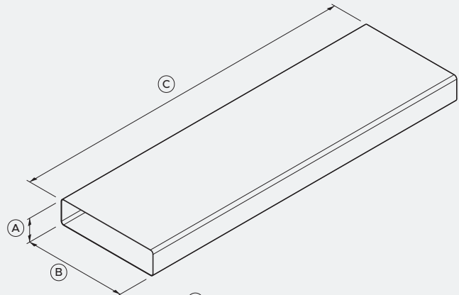
⑥ Duct 1M, 300x70
