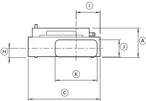
PROFILE VIEW
