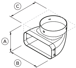
4 Adapter 90°, 150 to 222x89
