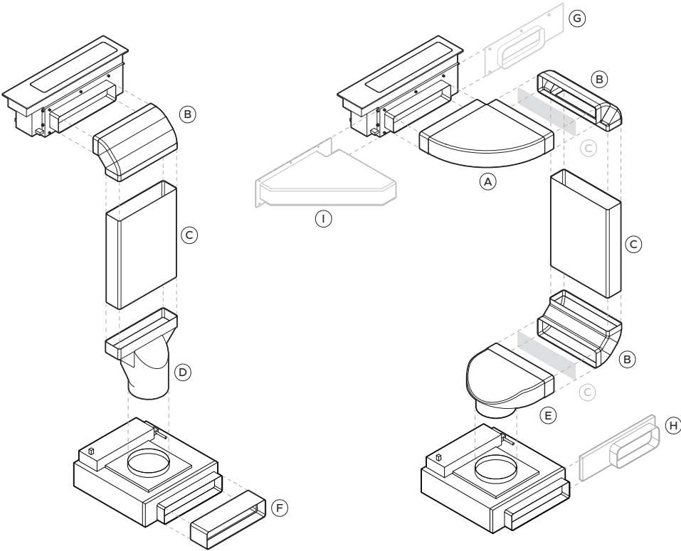
CD13DB1 CD13DG1 MODULAR DOWNDRAFT - 300 X 70 DUCTING
