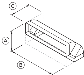
② Vertical Elbow 90°, 300x70
