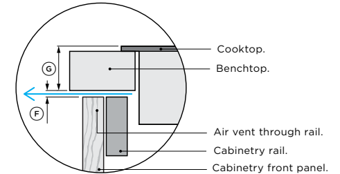
DETAIL 1 - PROFILE VIEW VENTILATION AT FRONT
