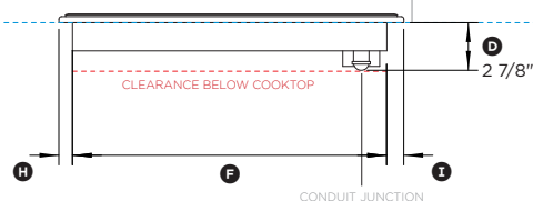
PROFILE VIEW
