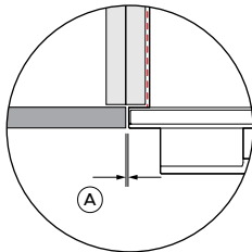
DETALJ 3 PLANVY
