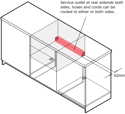
ISO VIEW
