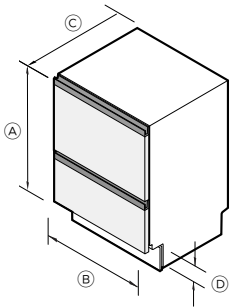
ISO VIEW
