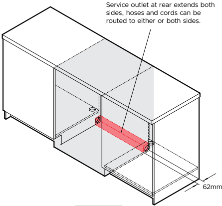
ISO VIEW
