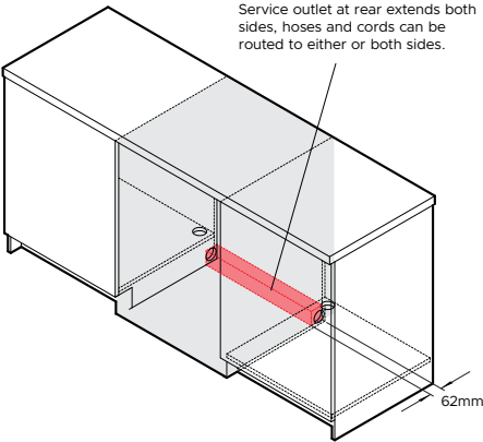
ISO VIEW
